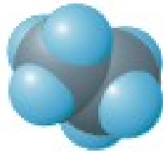
\text{C}_2\text{H}_6 Ethane
