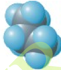
\text{C}_3\text{H}_8 Propane
